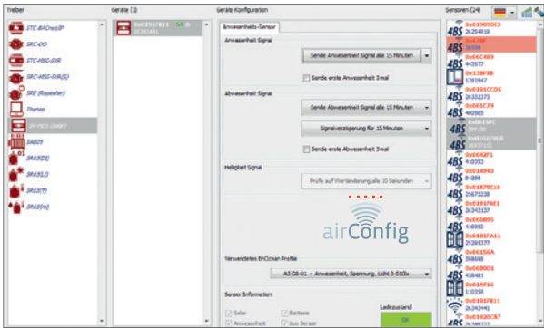
Parameterization of devices via Remote Commissioning
